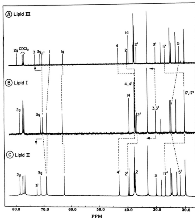
FIG. 4. ^{13}\text{C} NMR comparison between purified hydroxydiethers from M. barkeri and M. concilii , and diether. Lipids were isolated from TLC plates following hydrolysis of total polar lipids in 0.18% methanolic HCl for 24 h at 50 °C (see Fig. 3). Purity of the core lipids was confirmed by TLC. Spectra were recorded using \text{CDCl}_3 as solvent. Panel A, D OH( sn -2) from M. barkeri ; panel B, diether from M. barkeri ; panel C, D OH( sn -3) from M. concilii . Signal shifts are illustrated; g, glycerol.
