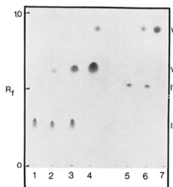
FIG. 7. Thin-layer chromatogram illustrating methylation rates for core lipids D_{OH(sn-2)} (III) and D_{OCH_3(sn-2)} (IV) of M. barkeri . Purified core lipids III and IV (see Fig. 1) were methylated by refluxing in CH_3I with Ag_2O as catalyst. Samples were removed for TLC analysis at various times. Lane 1, core lipid III; lanes 2-4, core lipid III methylated for 2, 5, and 29 h, respectively; lane 5, core lipid IV; lanes 6 and 7, core lipid IV methylated for 5 and 29 h, respectively.
