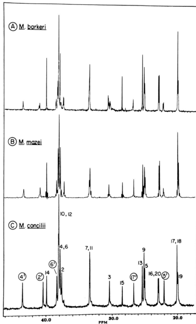
FIG. 2. ^{13}\text{C} NMR spectra of total polar lipids extracted from M. barkeri (A) and M. mazei (B). Purified digalactosylhydroxydiether (GalGalD OH ) from M. concilii (22) is shown as a reference (C). Signal assignments (8) are shown as carbon numbers primed to indicate origin from the sn -3 chain. In panel B, M. mazei was grown on ^{13}\text{CH}_3\text{OH}/^{12}\text{CH}_3\text{OH} (1:3.5, v/v). Polar lipids for A and B were prepared by acetone precipitation from the total lipid extracted from frozen-thawed cells (see "Experimental Procedures"). Spectra were recorded using benzene- d_6 /methanol- d_4 (7:2, v/v).
